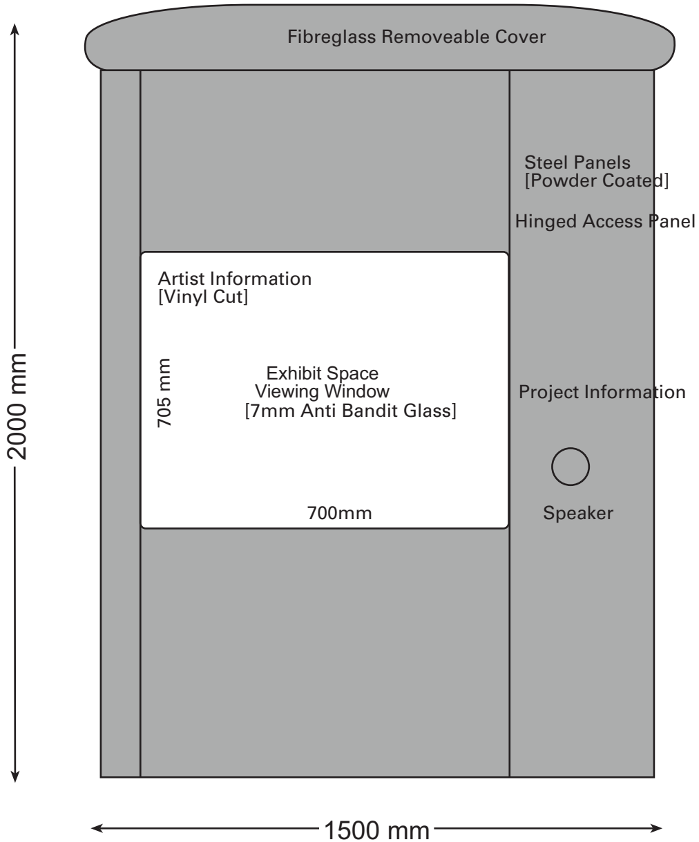
East - West Elevation* * Not to Scale
