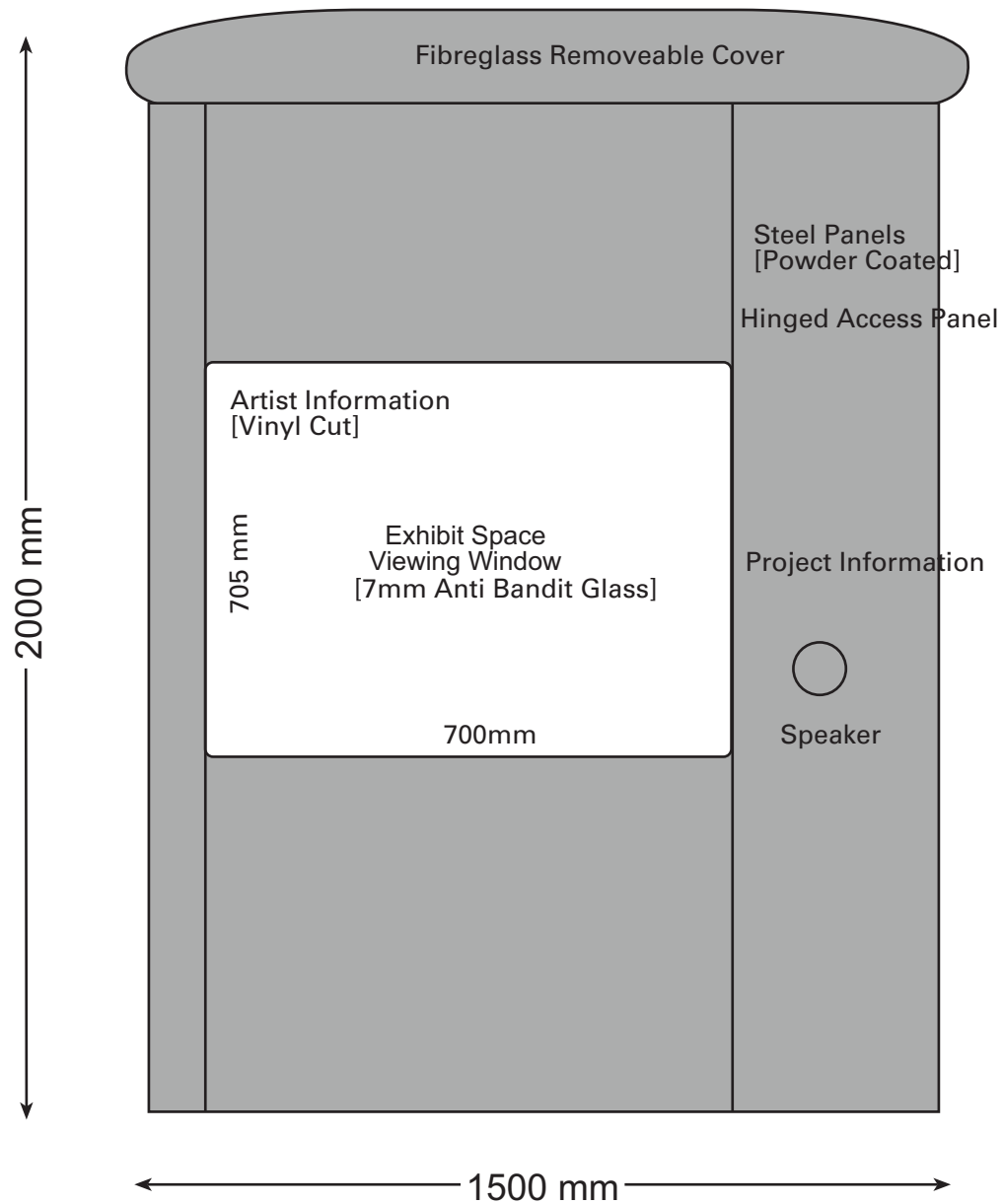
East - West Elevation* * Not to Scale
